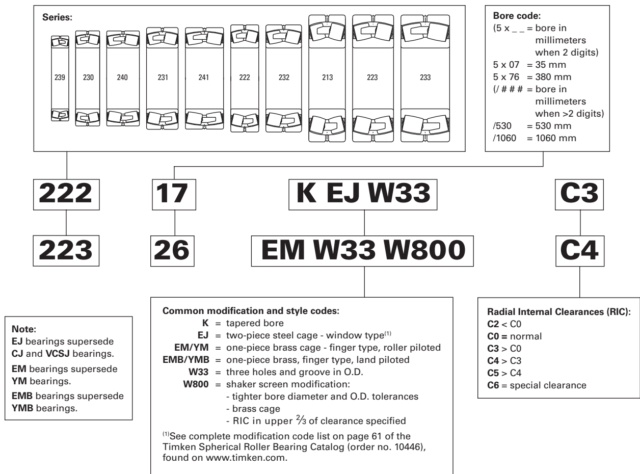
Fig. 35. Timken® spherical roller bearing nomenclature.
