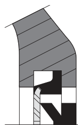
Fig. 15. V-ring seals.
