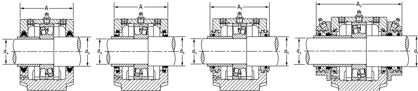
Double-Lip Seal
