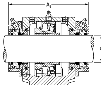
Taconite Seal
