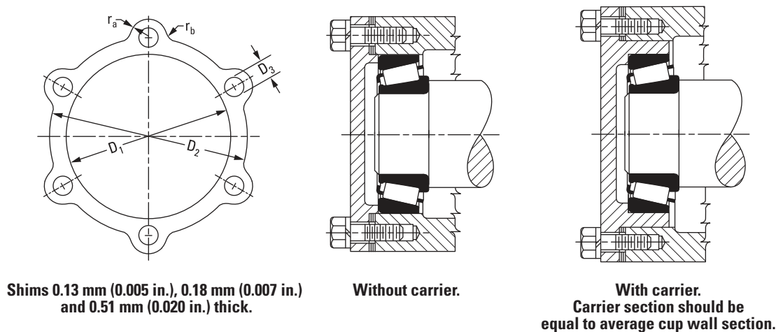
Fig. 57. Cup shims.
