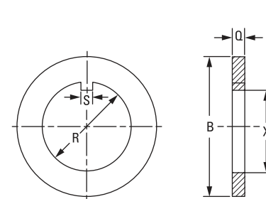
Fig. 51. Tongued washers.
