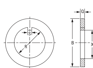
Fig. 54. Tongued washers.
