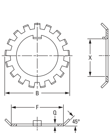
Fig. 50. Lockwashers.
